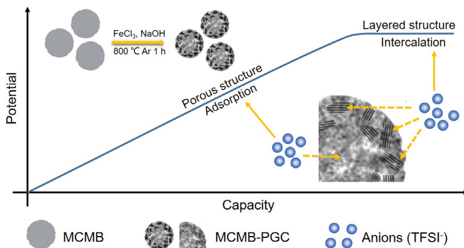
Fig. 1. Schematic diagram of the synthesis of MCMB-PGC and the dual-ion hybrid supercapacitor energy storage mechanism. Here MCMB denotes mesocarbon microbeads and PGC denotes porous graphitic carbon.
