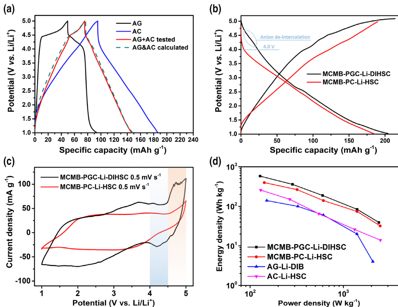
Fig. 4. (a) GCD curves of AG, AC, a mixture of AG and AC, and the calculated curve by weighted average under 0.1 A g -1 ; (b) GCD curves of a MCMB-PGC-based Li-DIHSC and a MCMB-PC-based Li-HSC under 0.1 A g -1 ; (c) CV curves of MCMB-PGC-based Li-DIHSC and MCMB-PC-based Li-HSC under 0.5 mV s -1 ; (d) Ragone plots of the as-fabricated devices. Here AG denotes artificial graphite; AC denotes activated carbon; HSC denotes hybrid supercapacitor; DIB denotes dual-ion battery; DIHSC denotes dual-ion hybrid supercapacitor.
