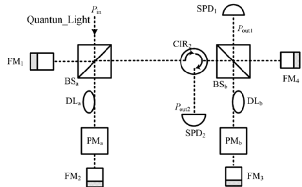
Figure 1 Simplified light path of F-M system. BS, 50/50 beam splitter; FM, Faraday mirror; SPD, single photon detector; CIR, circulator; DL, fiber delay line.
